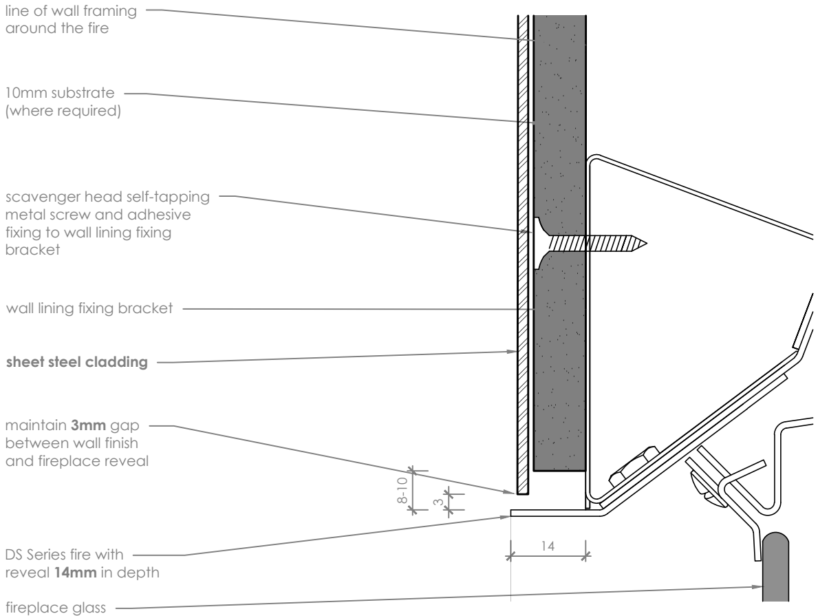
Finish Detail
