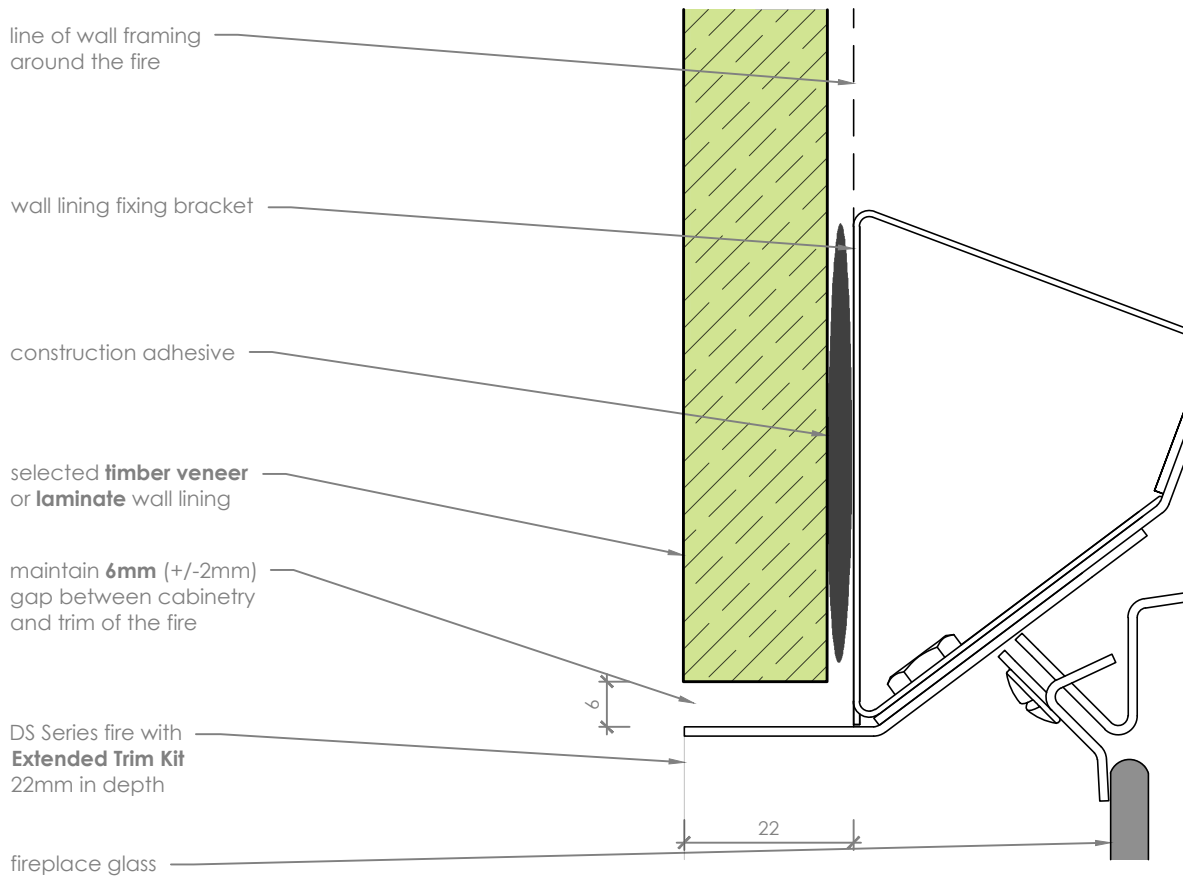
Cabinetry Detail
