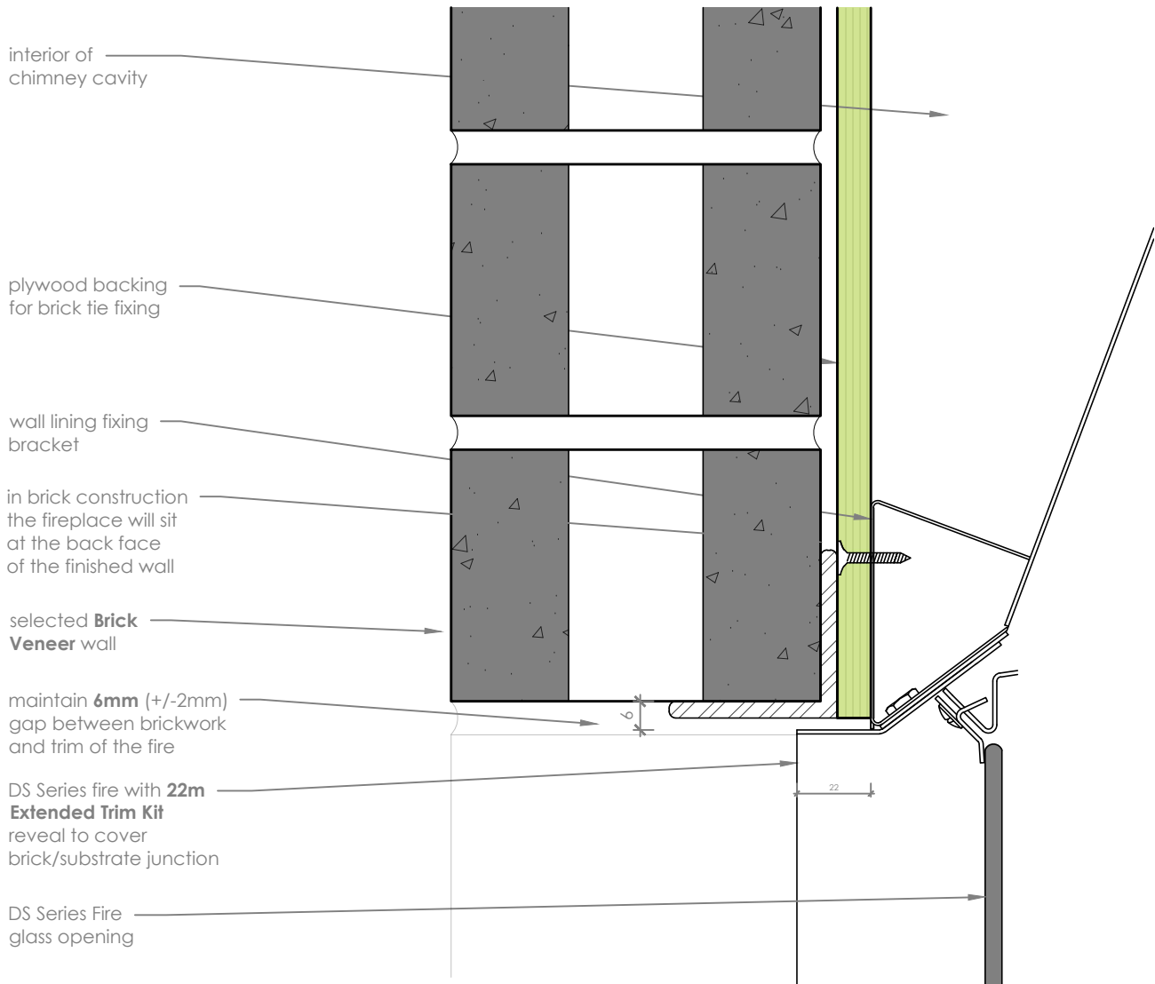
Brick Veneer Detail
