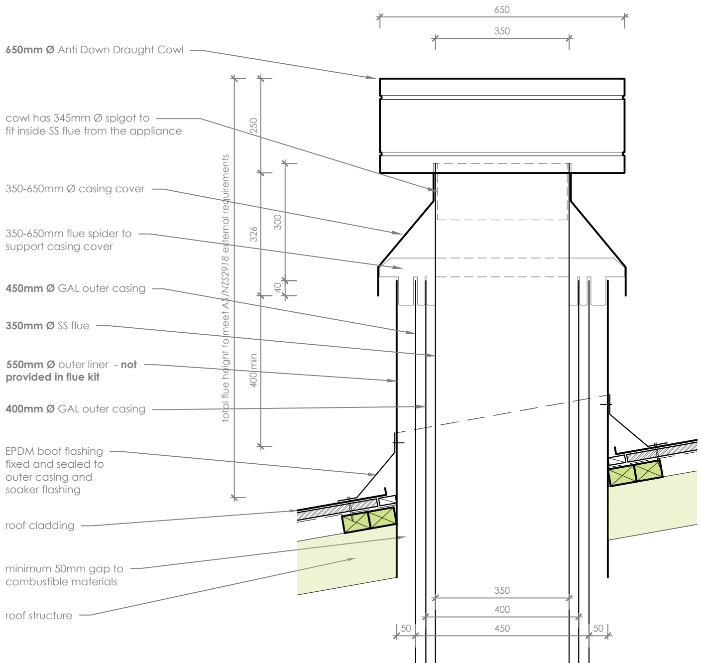
Roof Penetration Detail
